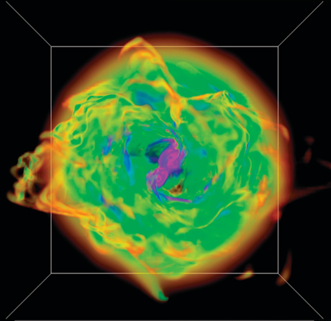
Volume rendering of the gas density in a simulation of the formation of a 70 Solar mass binary system. Krumholz
